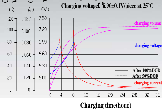
Charging characteristics Charging voltage \pm 0.1V /piece at 25°C
