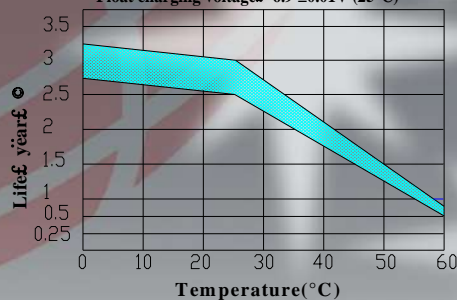
Temperature effect on float life Float charging voltage \pm 0.01V (25°C)
