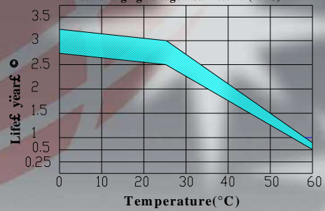
Temperature effect on float life Float charging voltage: 6.9 \pm 0.01V (25°C)
