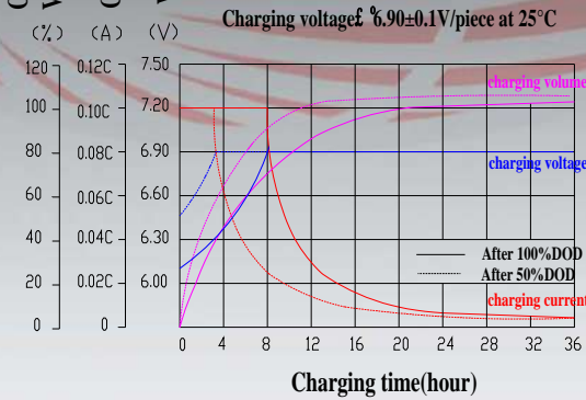
Charging characteristics Charging voltage: 6.90 \pm 0.1V /piece at 25°C
