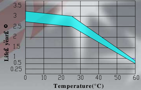
Temperature effect on float life Float charging voltage: 6.9 \pm 0.01V ( 25^{\circ}C )
