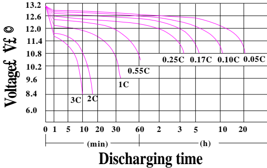
Discharge characteristics ( 25^{\circ}C )
