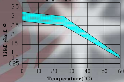
Temperature effect on float life Float charging voltage \%6.9 \pm 0.01V (25°C)
