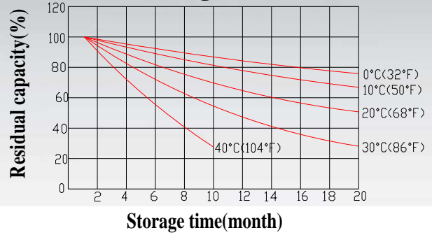
Temperature effect on battery self-discharge
